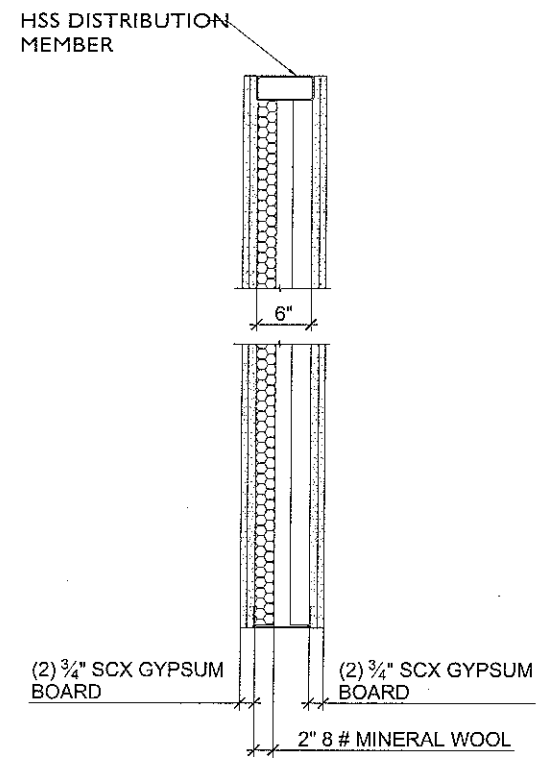
INTERIOR INTEGRITY WALL FOUR HOUR FIRE RATED
