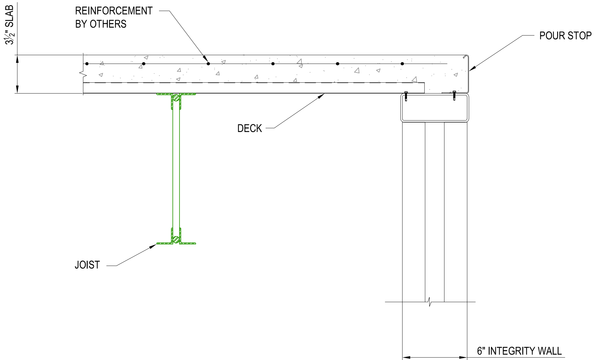
DECK BEARING DETAIL
